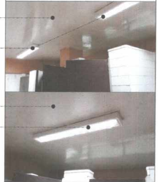
Existing plywood ceiling board to be removed and replaced with standard 6mm marine plywood, painted finished Existing lighting fixtures to be retained
