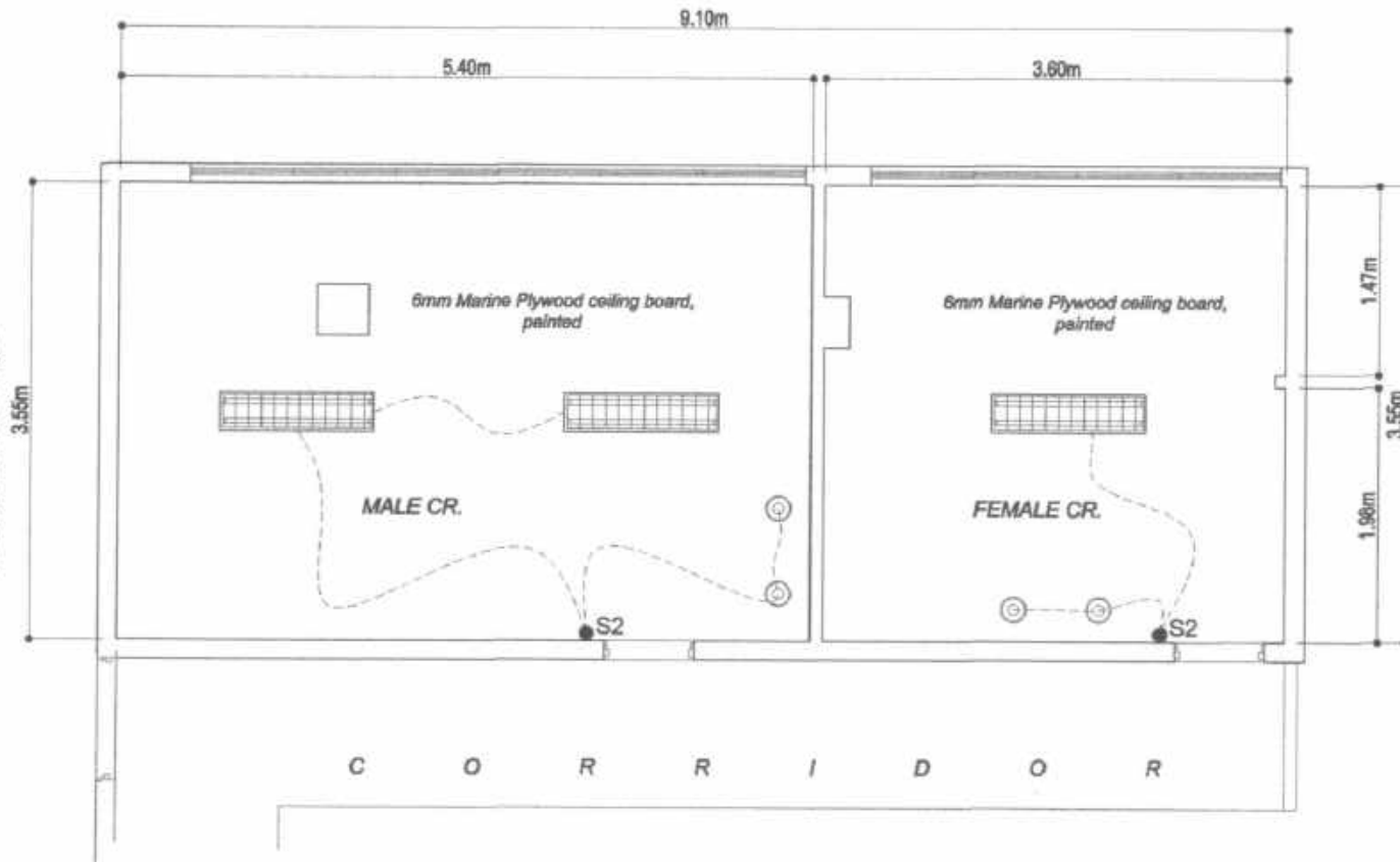
1 ELECTRICAL LIGHTING LAYOUT SCALE 1 : 60 MTS
