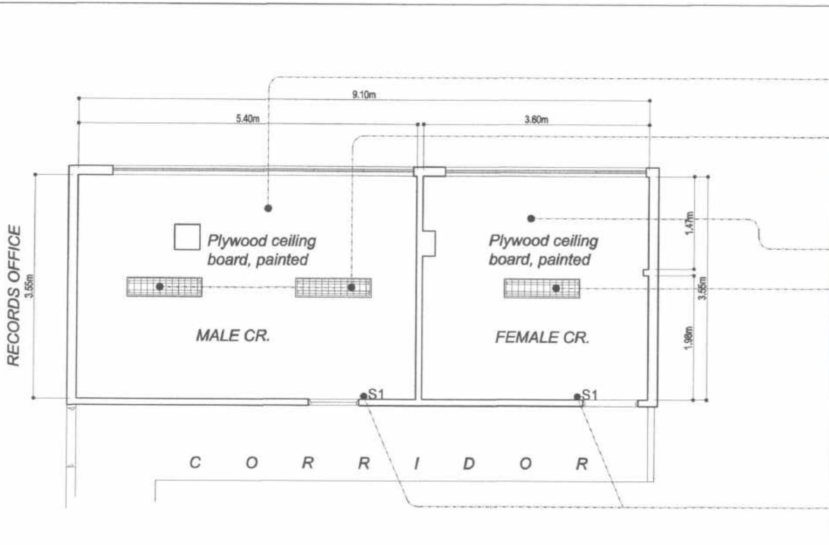
1 REFLECTED CEILING PLAN (As-built) A/4 SCALE 1:60MTS
