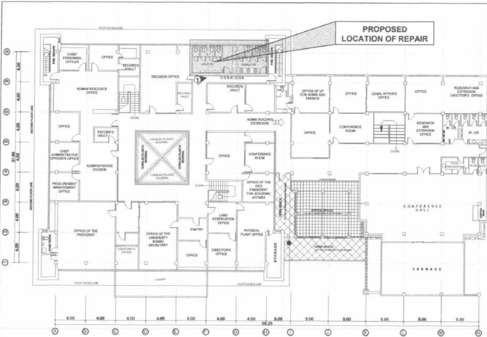
1 SECOND FLOOR PLAN (Administration Building) SCALE 1:300MTS
