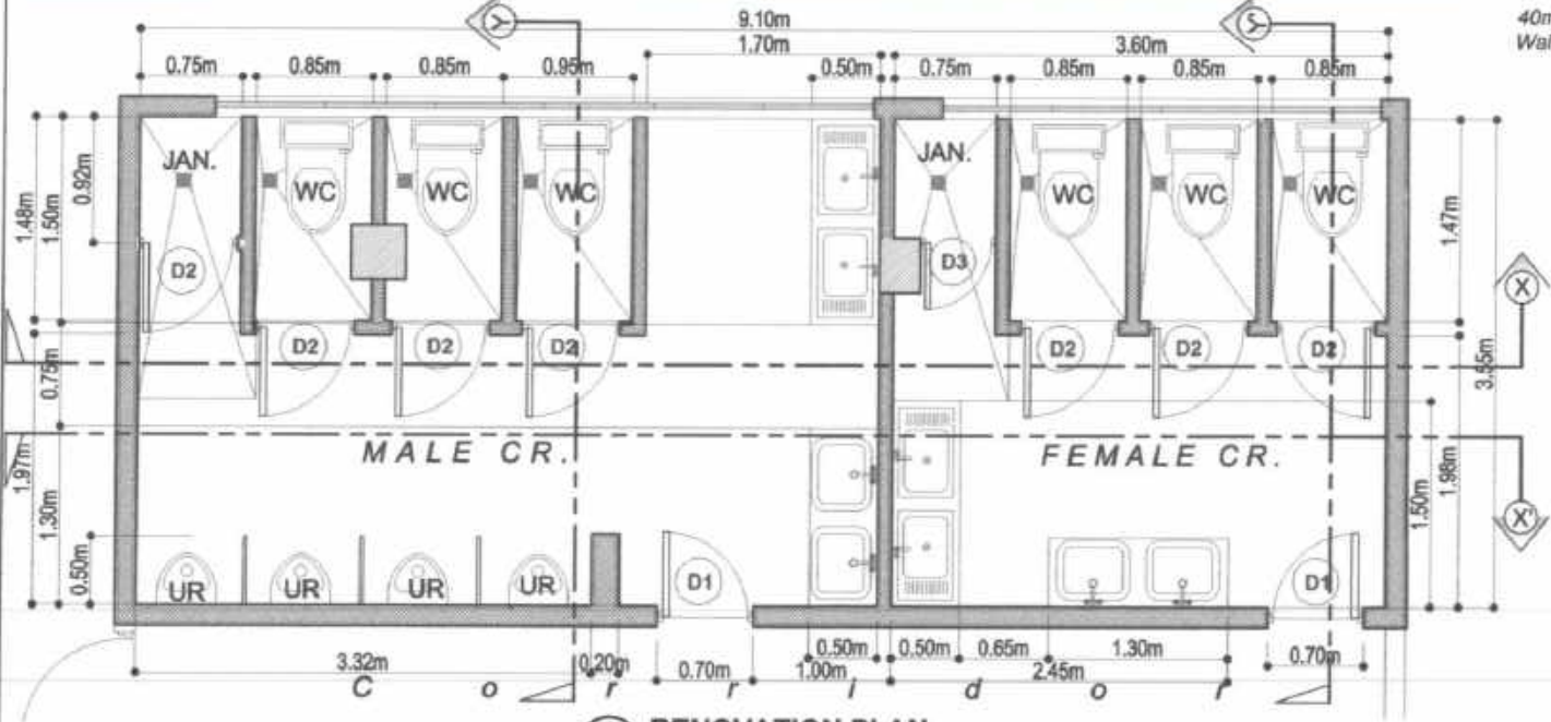
1 RENOVATION PLAN SCALE 1:60MTS
