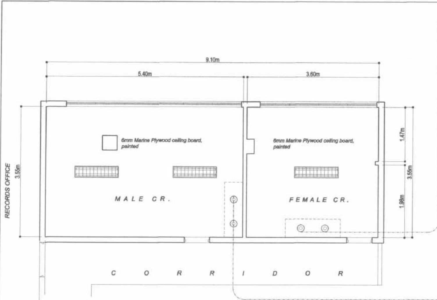
1 REFLECTED CEILING PLAN (Renovation) SCALE 1:80MTS
