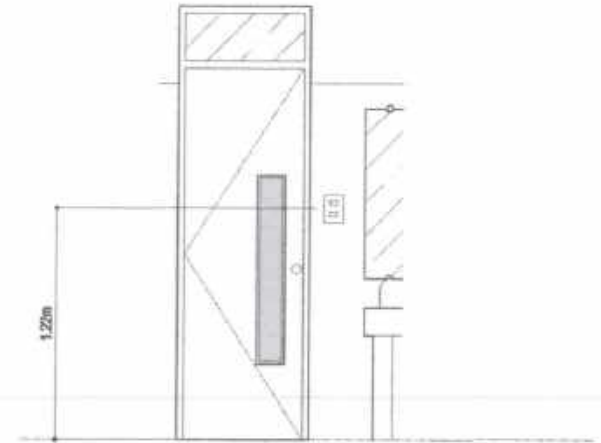
2 MOUNTING HEIGHT SCALE 1:40MTS
