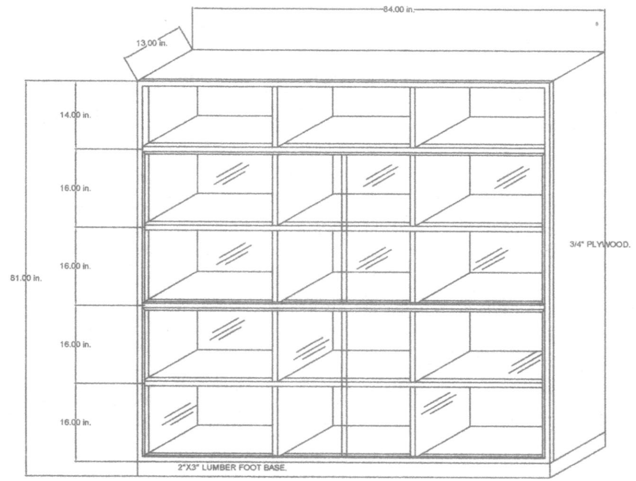
1-UNIT WOODEN CABINET W/ 1/4" CLEAR GLASS SLIDING DOOR.
