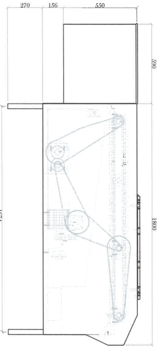
TOP VIEW
