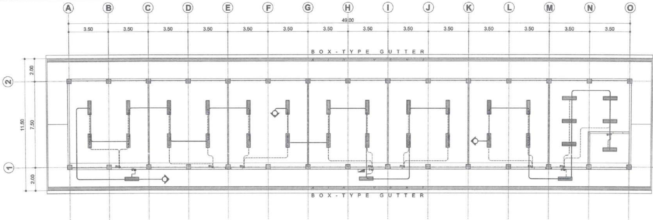
1 E 1 ELECTRICAL LIGHTING LAYOUT SCALE 1 : 200 MTS
