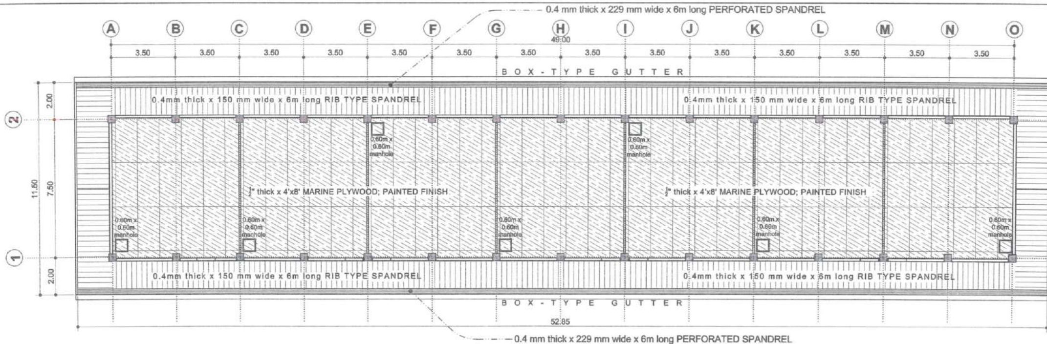
1 A-3 REFLECTED CEILING PLAN SCALE 1 : 200 MTS
