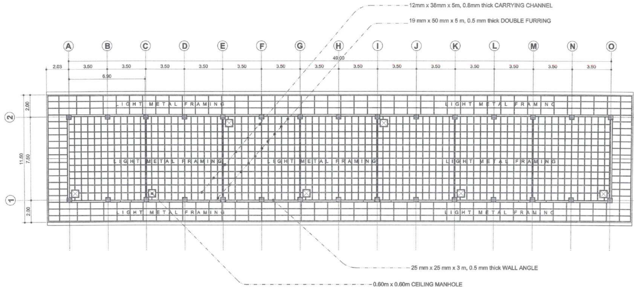
1 A 4 CEILING FRAMING PLAN SCALE 1 : 200 MTS
